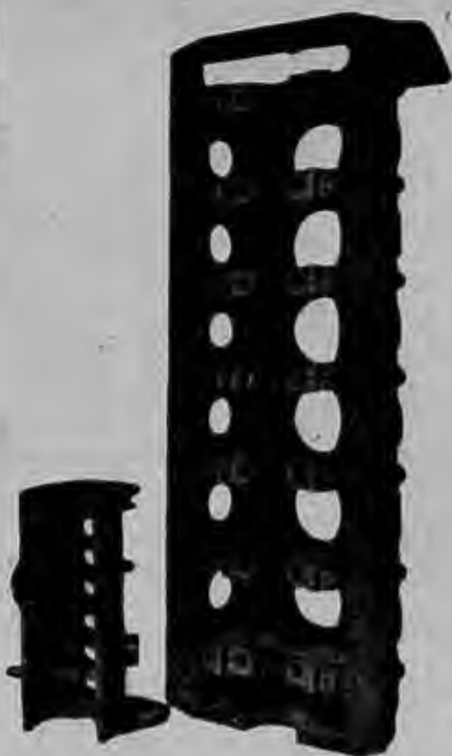
Fig. 1a.—Large Diesel-engine crankcase cast in Elektron magnesium alloy. The overall sizes are 8 ft. x 3 ft. 3 in. x 1 ft. 6 in. and the weight 6 cwt. In aluminium alloy the weight of a similar crankcase is approximately 10 cwt. The crankcase on the left, shown for comparison, is for a 25 h.p. motor car engine.
